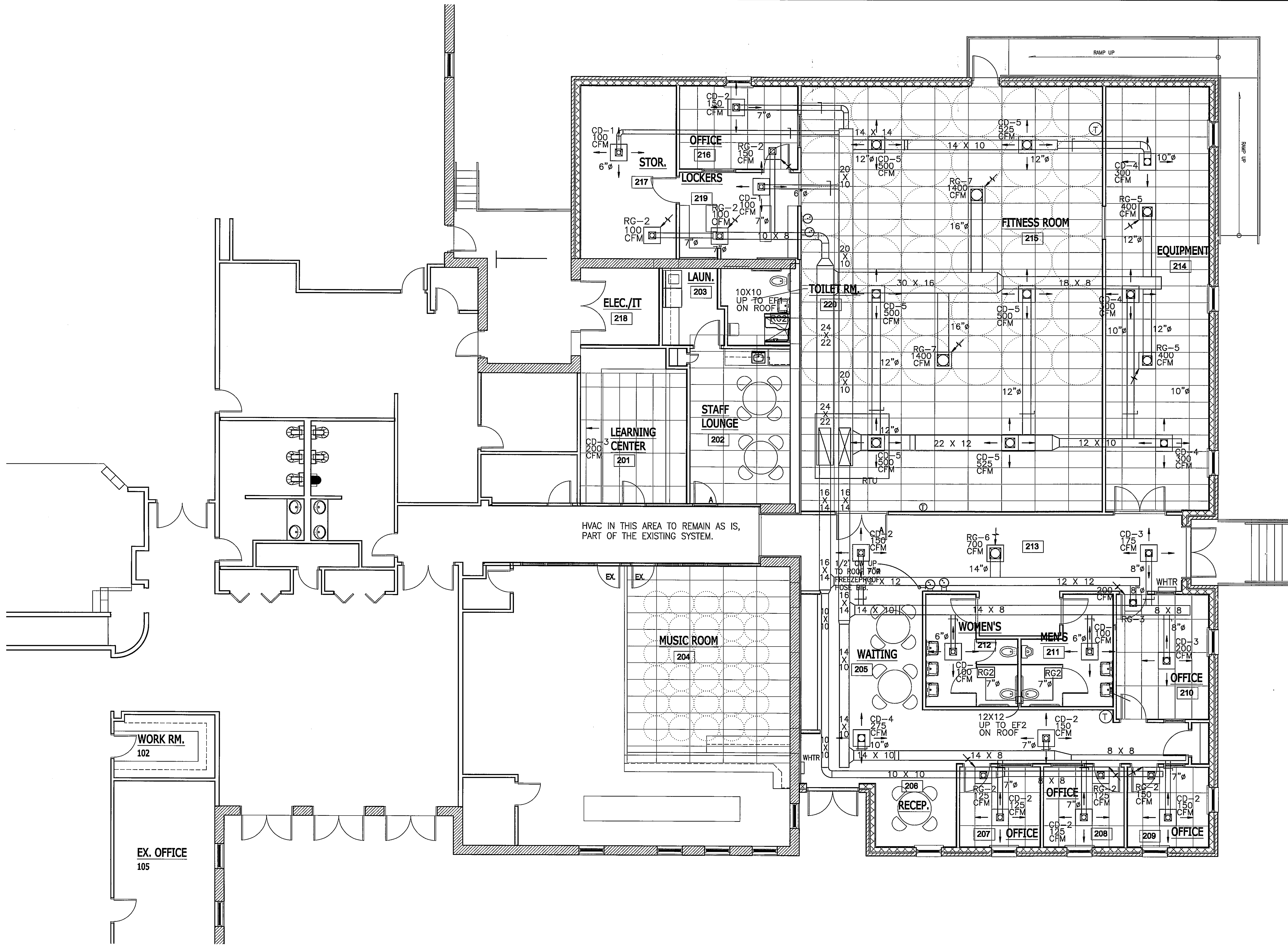
MECHANICAL PLAN 1/8"=1'-0"
