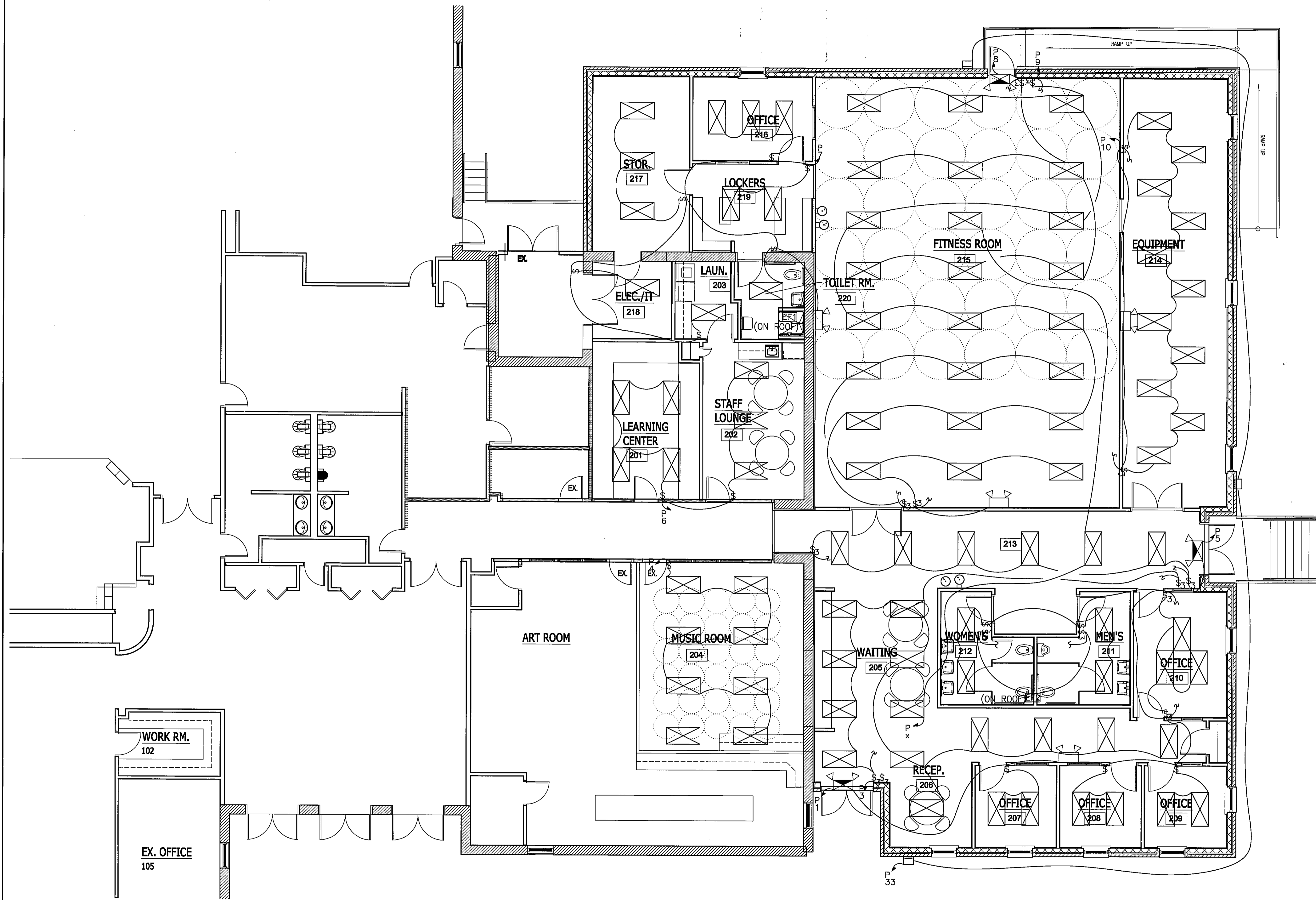
LIGHTING PLAN 3/16"=1'-0"
