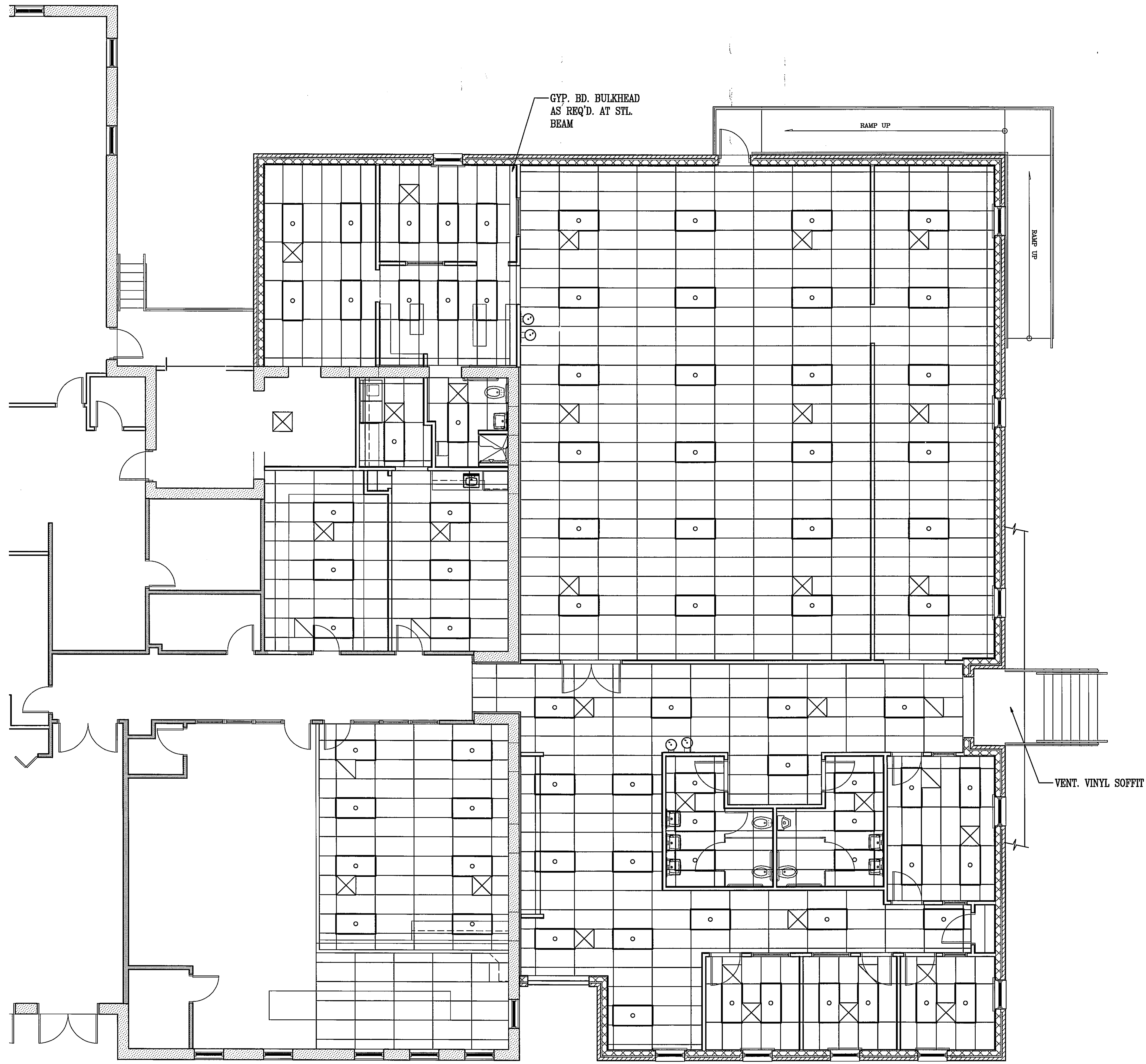
1 REFLECTED CEILING PLAN 3/16" = 1'-0"
