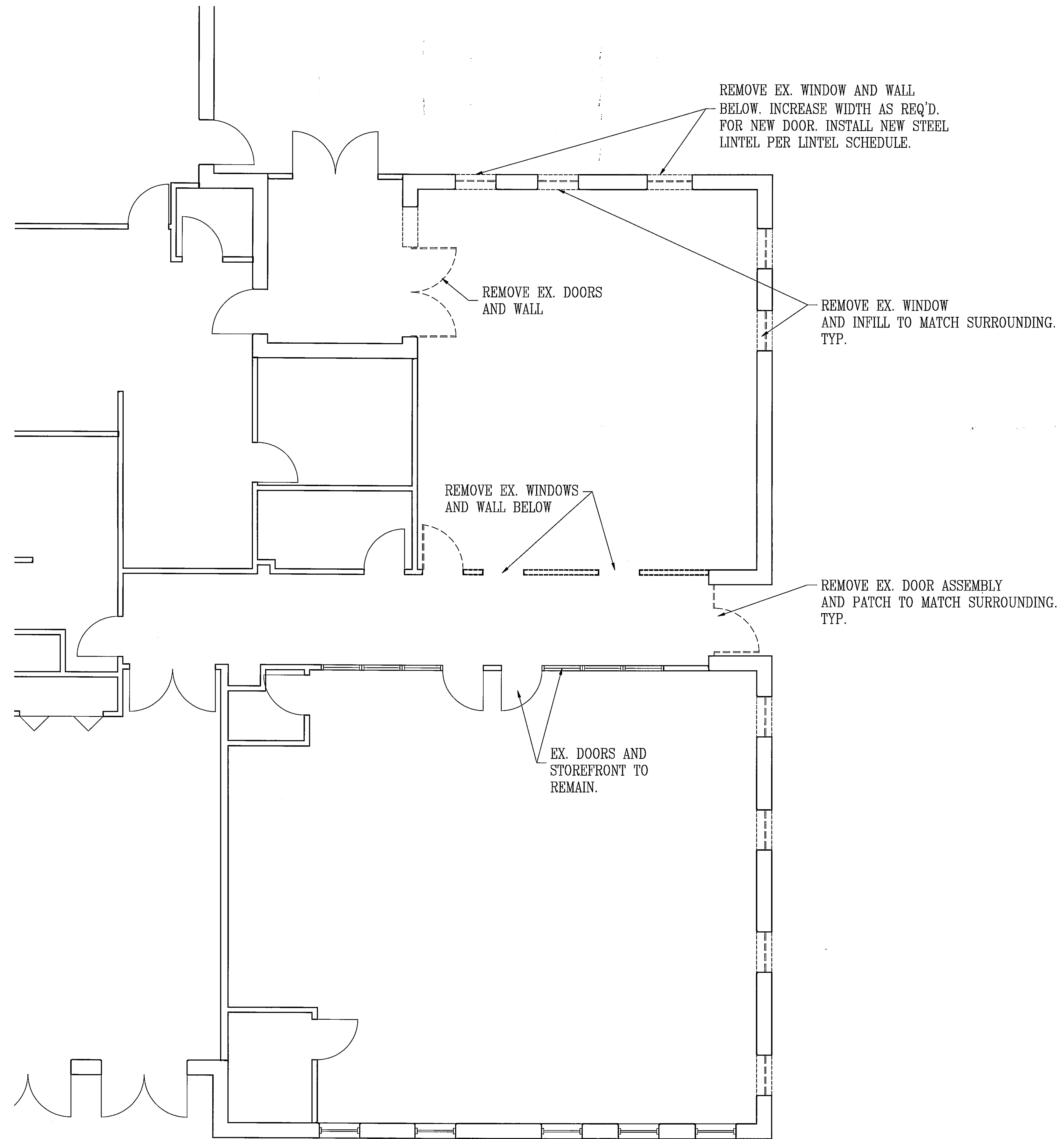
1 DEMOLITION PLAN 1/4"=1'-0"
