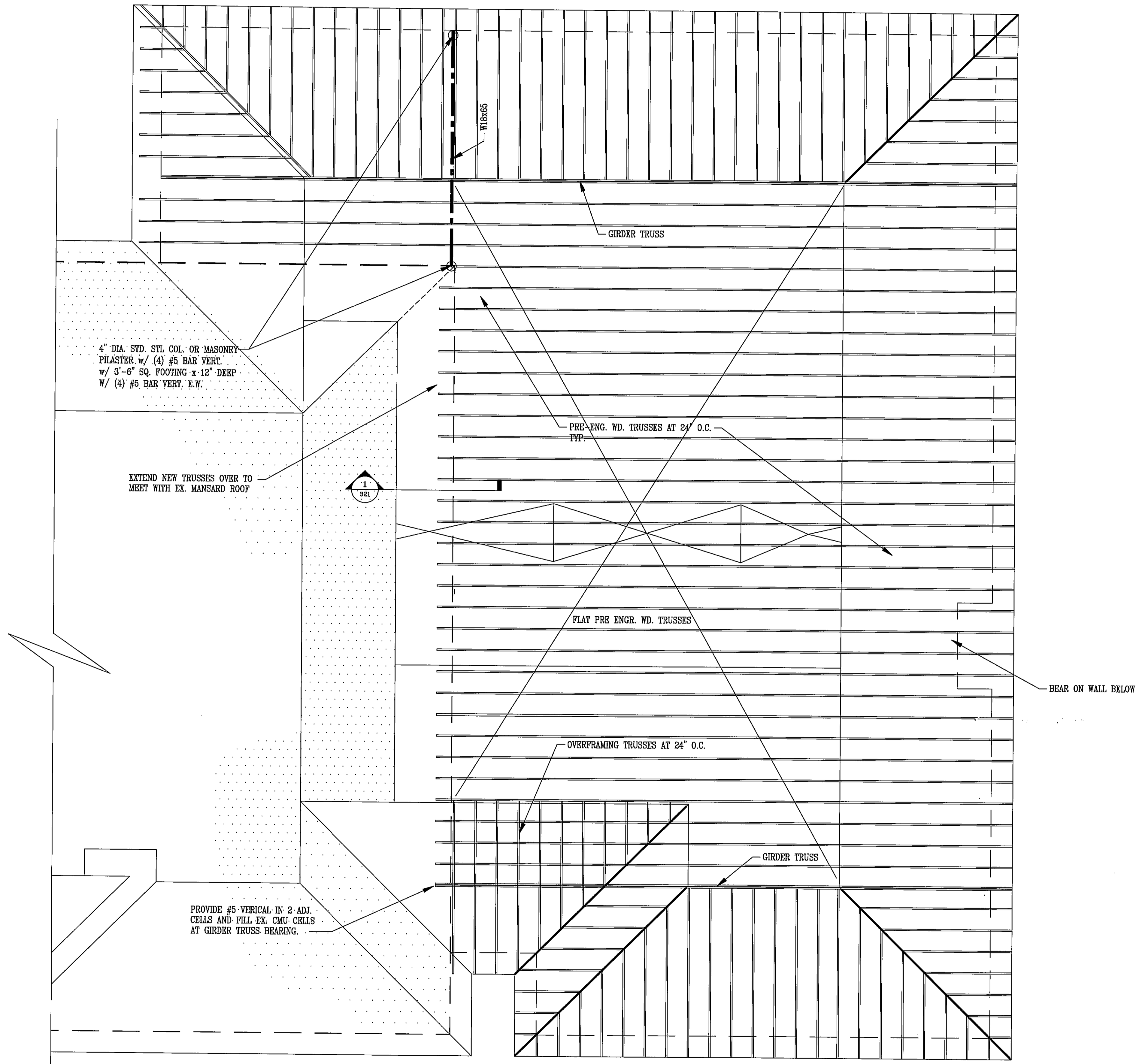
1 ROOF FRAMING PLAN 3/16-1-5
