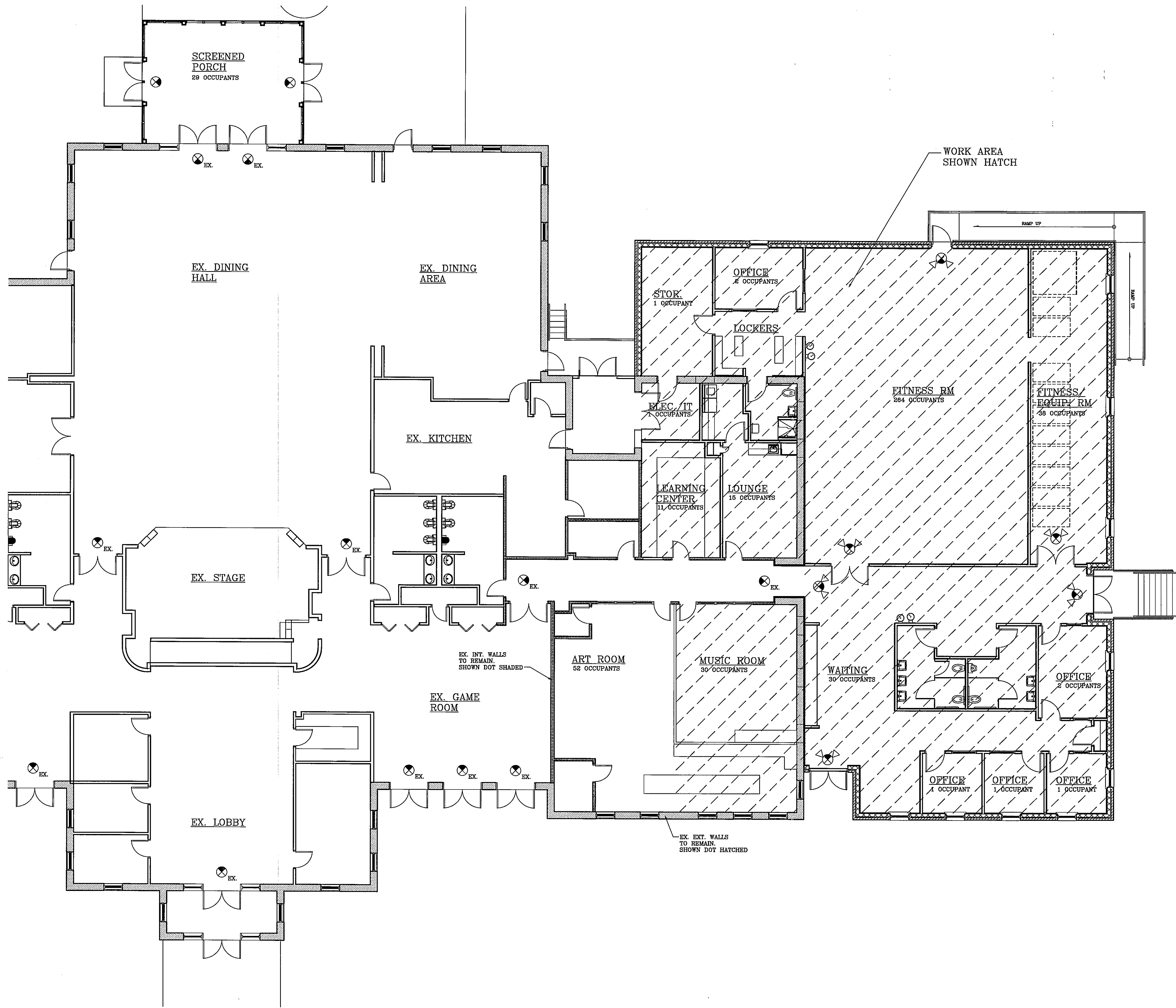
① FIRE RATING AND EGRESS PLAN SCALE: 1/8" = 1'-0"
