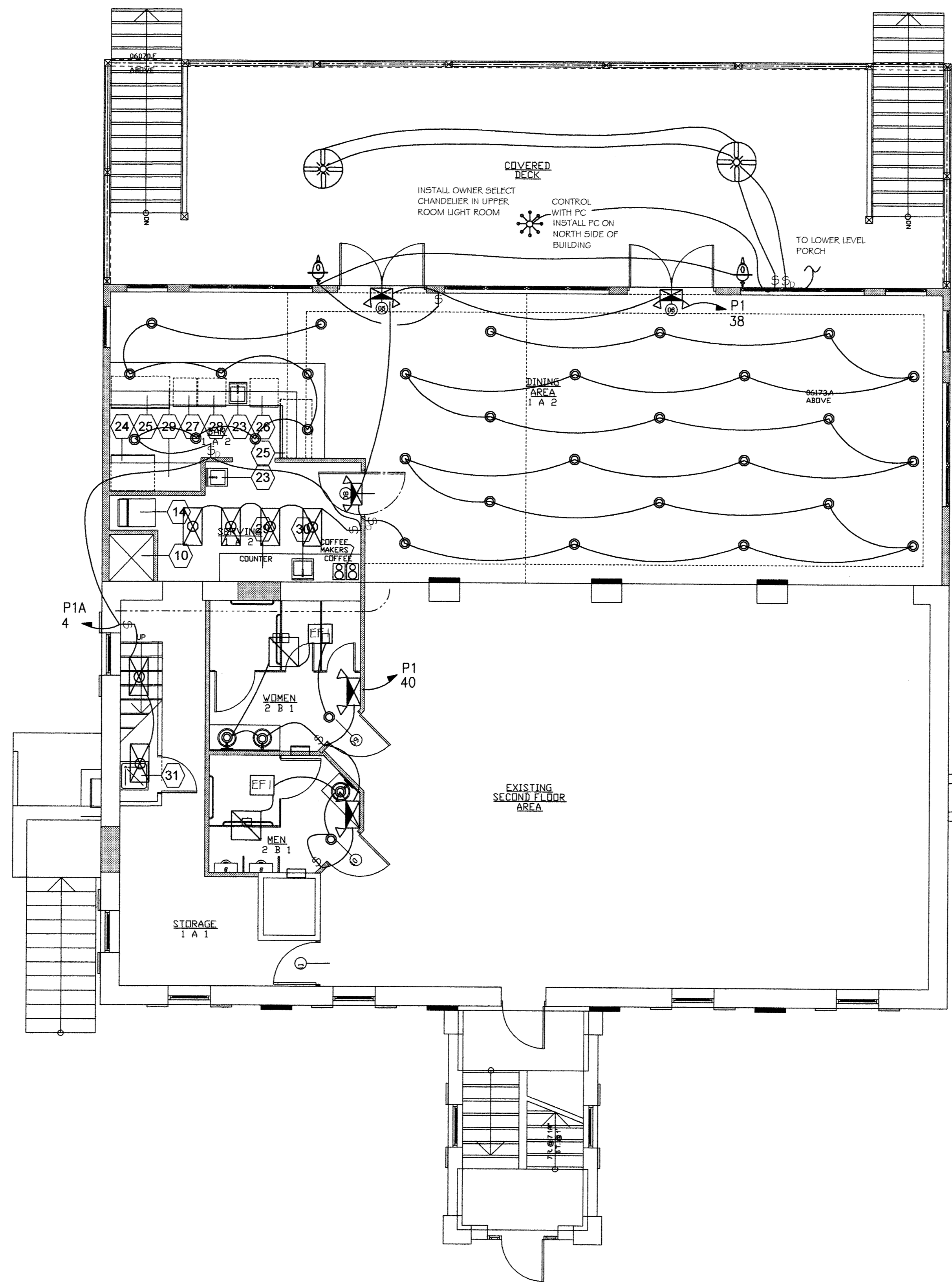
UPPER LEVEL LIGHTING PLAN
